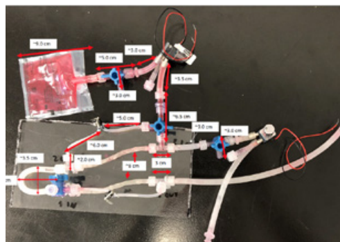
Figure 2 : Circuit hydraulique
